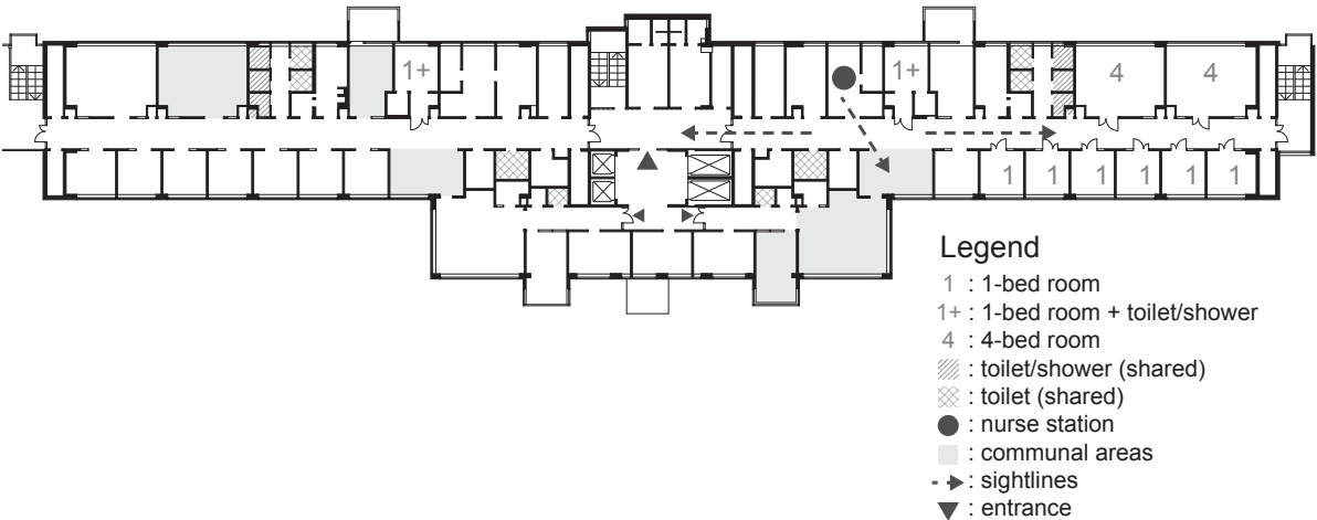
Fig. 7. One ward in Old hospital. The floor layout is corridor-based, enabling observation of bedroom doors and doors of most shared toilets and showers but not most seating areas and activity rooms. Ward group size at 100% occupancy = 16 patients. Scale 1:500.
